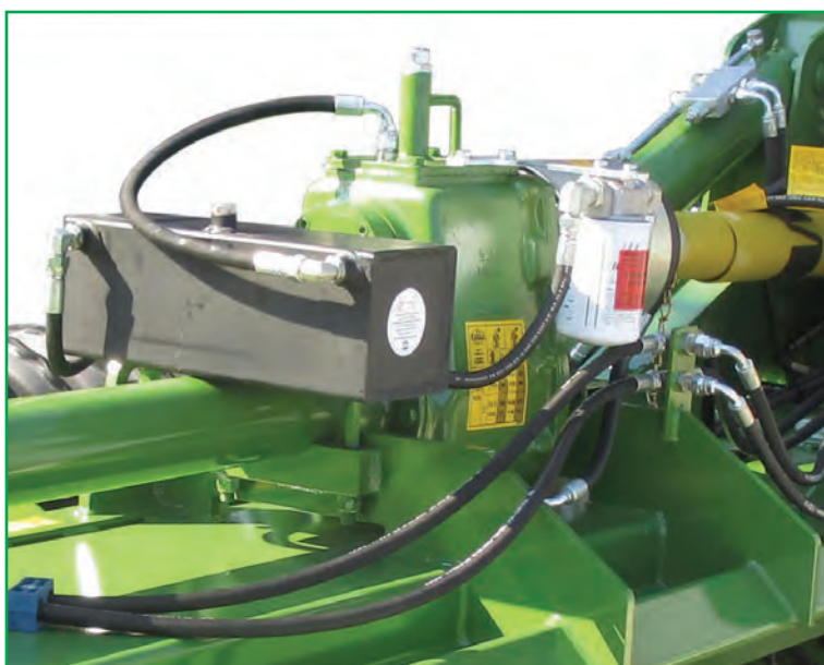
Oil cooling kit for side gearboxes with reservoir (optional)
