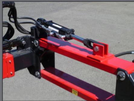
PARALLEL LINKAGE
