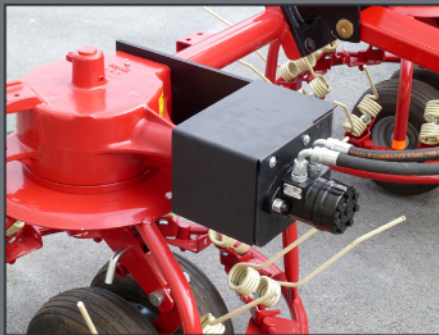
DT-SIT MOUNTING
